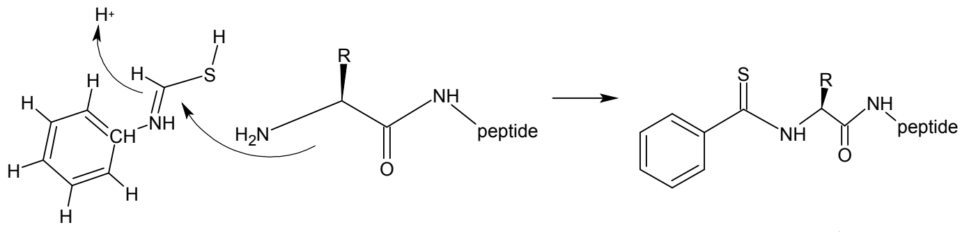
Phenylisothiocyanate
