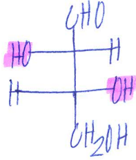
(-)-D-Threose
