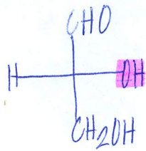
(+)-D-Glyceraldehyde
