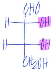
(-)-D-Erythrose
