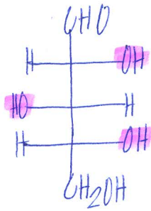
(+)-D-Xylose
