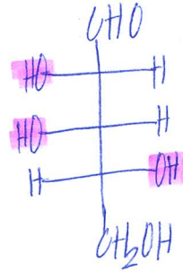
(-)-D-Lyxose
