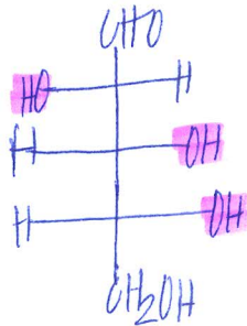
(-)-D-Arabinose
