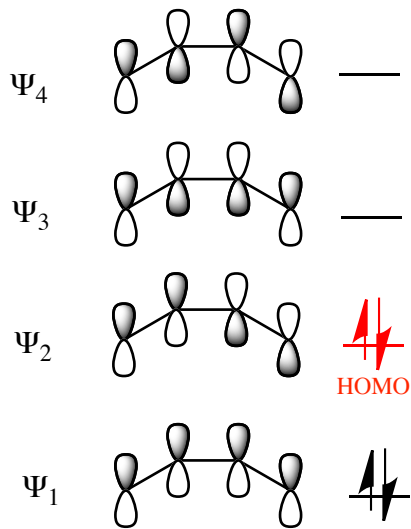
\pi -system molecular orbitals
