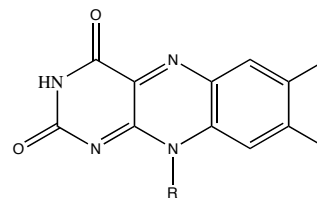
riboflavin
