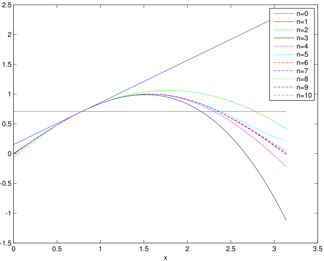
Taylor series expansion for f(x)=\sin(x) at x_0=\pi/4 for n=0,1,\dots,10
