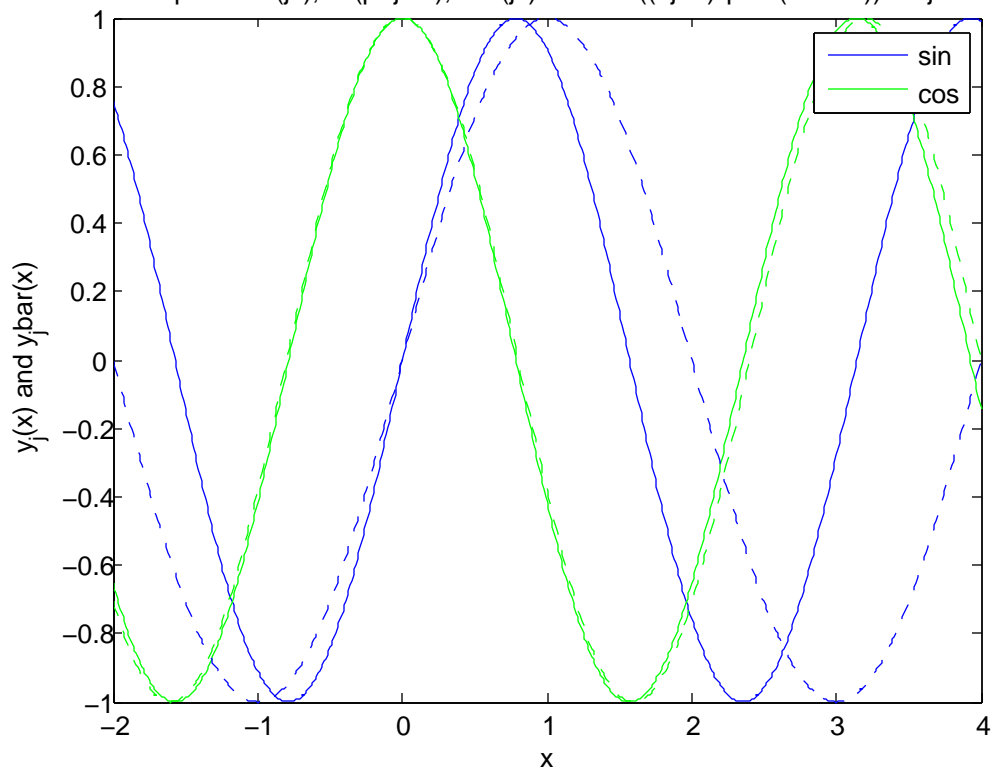
Graph of \sin(jx) , \sin(\pi*jx/4) , \cos(jx) and \cos((2j+1)*\pi*x/(2*\beta)) for j=2
