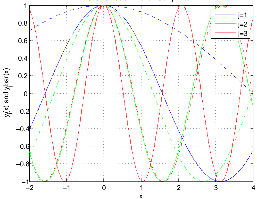
Cosine Basis Function Comparison
