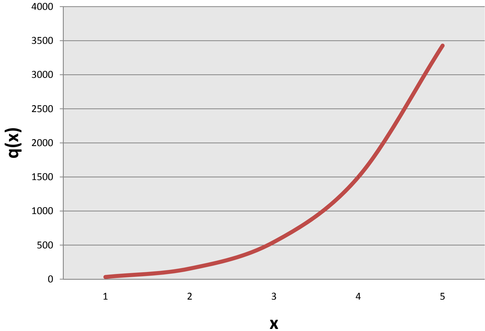
Figure 2 q(x)=a_iP_i(x)
