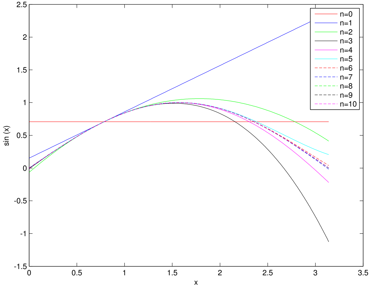
Taylor series expansion for f(x)=\sin(x) at x_0=\pi/4 for n=0,1,\dots,10
